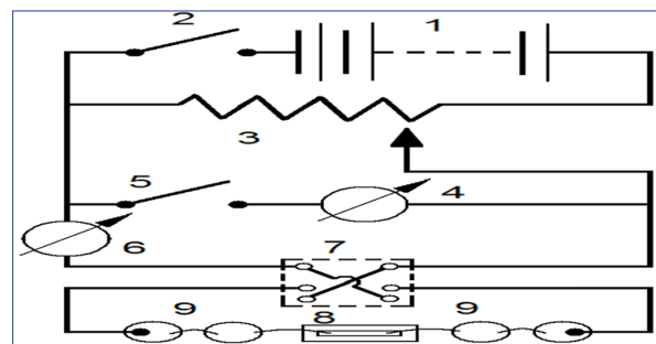
Figure 4: Electrical circuit diagram of the electrophoresis system.
